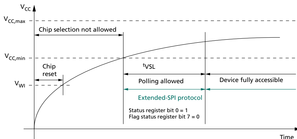
Figure 47: Power-Up Timing
