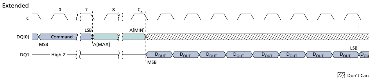
Figure 18: READ – 03h/13h 3
