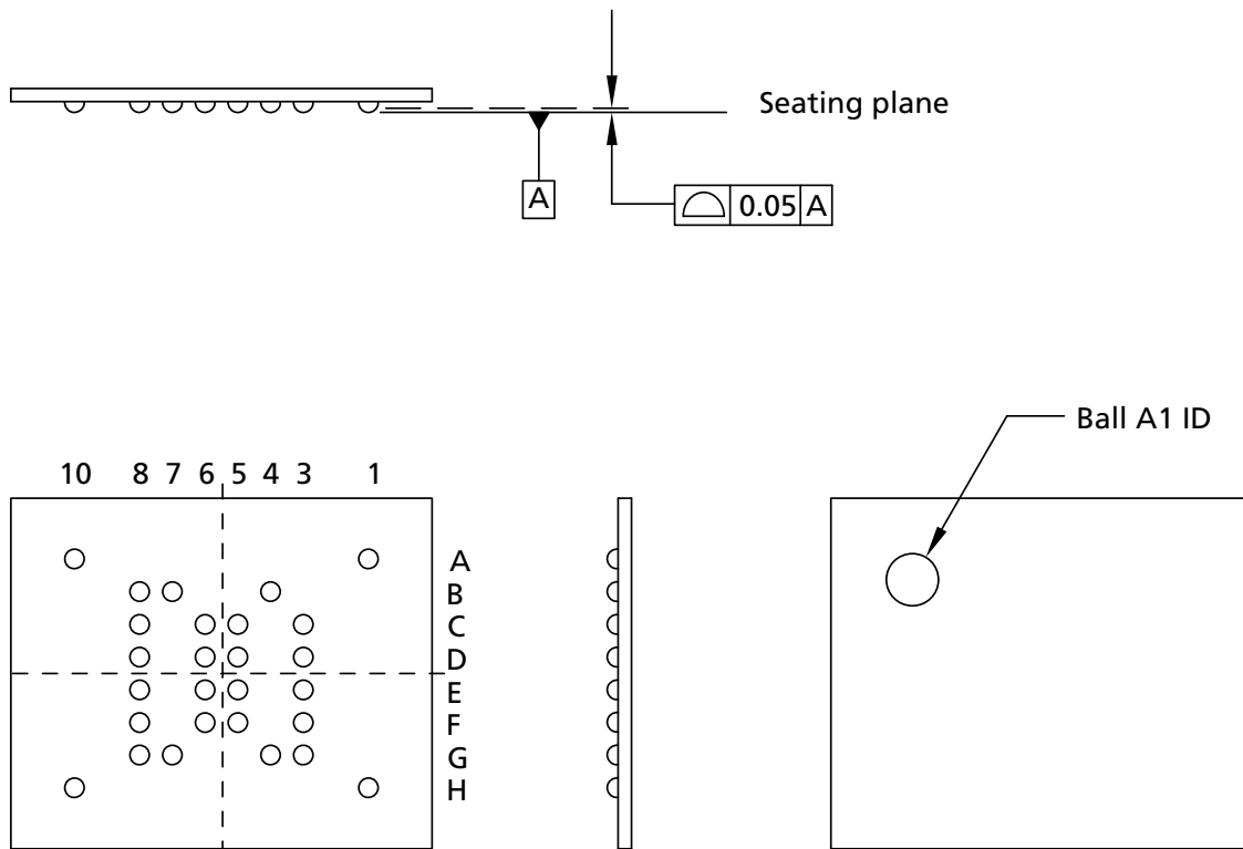
Figure 9: 27-Ball XFWLBGA
