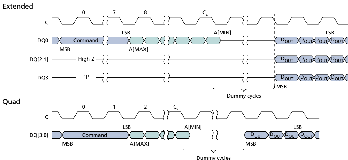
Figure 28: DTR QUAD OUTPUT FAST READ – 6Dh 3
